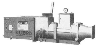
MODEL 800 VACUUM DEAIRING PUGMILL 1000 Pounds per Hour
