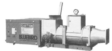
MODEL 800 VACUUM DEAIRING PUGMILL 1000 Pounds per Hour
