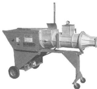
MODEL 3000 HEAVY DUTY PUGMILL 2000 Pounds per Hour
