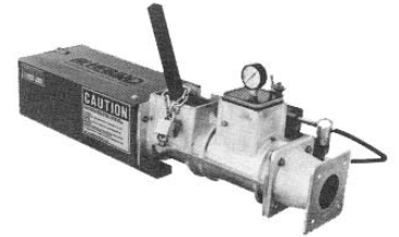
MODEL 440 VACUUM DEAIRING PUGMILL 350 Pounds per Hour
