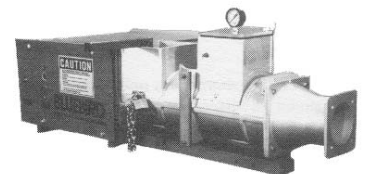
MODEL POWERSTAR-1 VACUUM DEAIRING PUGMILL 1200 Pounds per Hour
